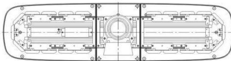
TBD-280003: 3pcs*3w/pc for a group, totally 22 groups , and speaker in center
